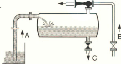
Use of gas jet vacuum pump for elevation of liquids
